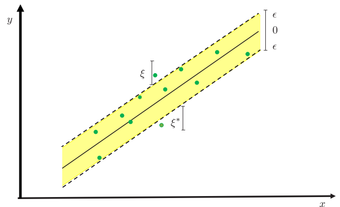
Figure 6: Support vector regression illustration.
