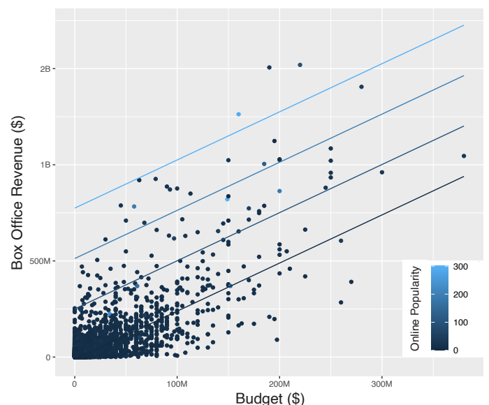
Figure 1: Multi-linear regression example using budget and online popularity obtained using data from The Movie Database [3].
