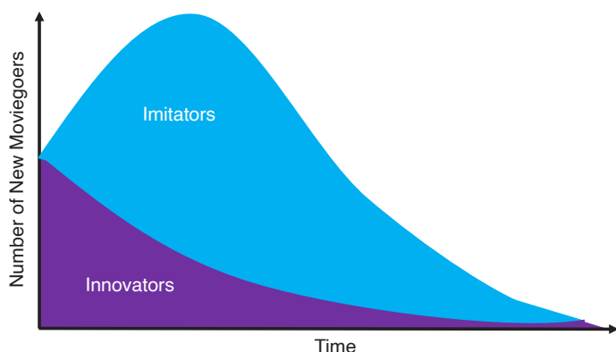
Figure 2: Bass diffusion model, illustration of new moviegoers.
