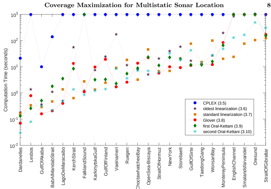
FIGURE 2. Comparison of the solution time for all model formulations and all instances (sorted by increasing solution time for the respective fastest run).
