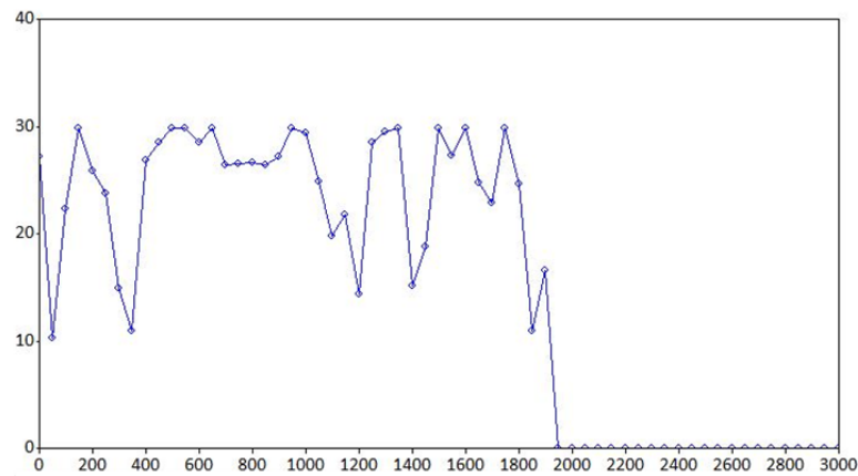
Fig. 2. Velocity (in m/s) over time (in s) in the solution to instance #6.
