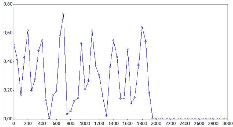
Fig. 3. Acceleration (in \text{m/s}^2 ) over time (in s) in the solution to instance #6.
