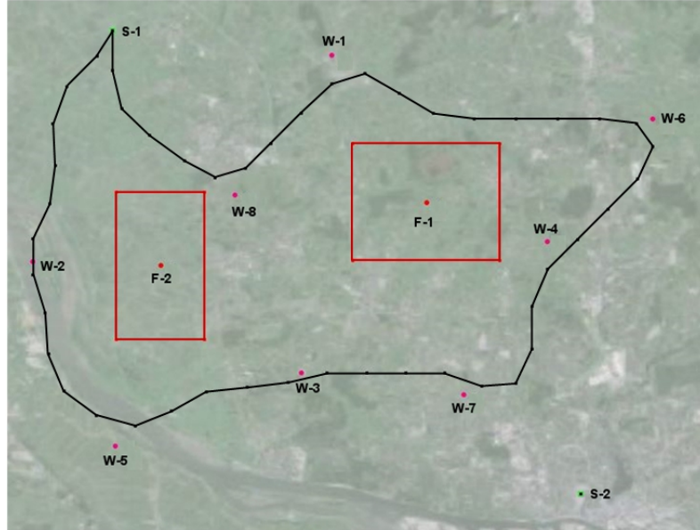
Fig. 1. Visualization of the solution to instance #6. S-1, S-2 are the start/end locations for the UAV's trajectories. W-1, ..., W-8 are the waypoints. F-1, F-2 are restricted airspaces. (Background image source: GoogleMaps.)
