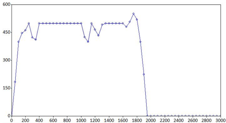
Fig. 4. Altitude (in m) over time (in s) in the solution to instance #6.
